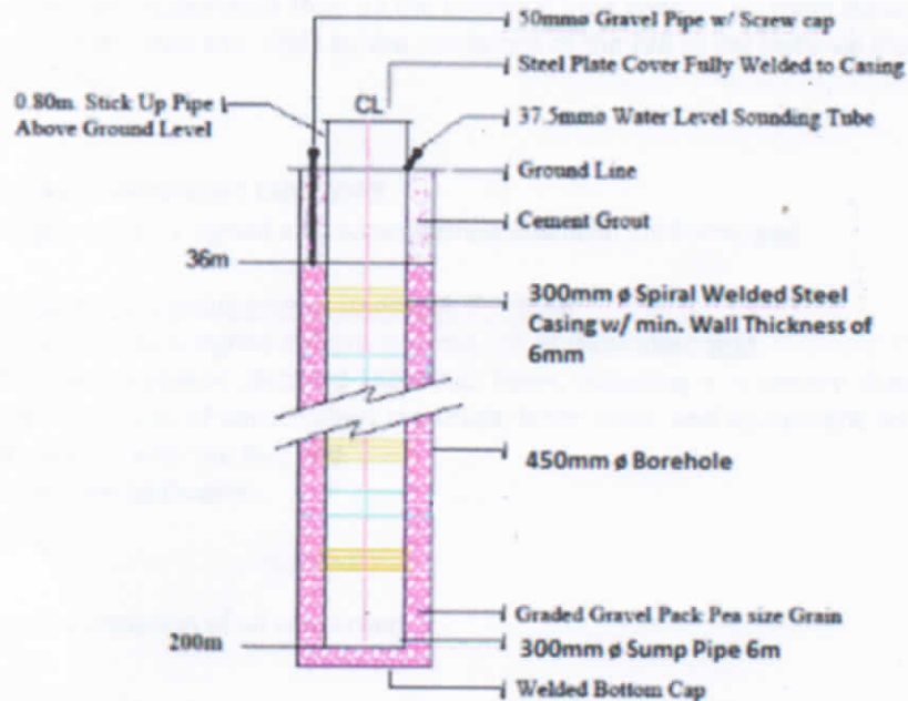
PRELIMINARY WELL DESIGN
